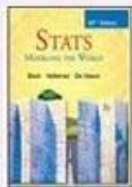
AP Statistics
